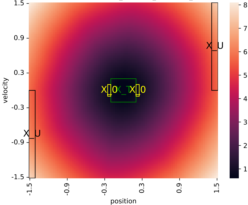
Learned certificate (2026-06-01_05-33-28_certificate_iteration=2)
