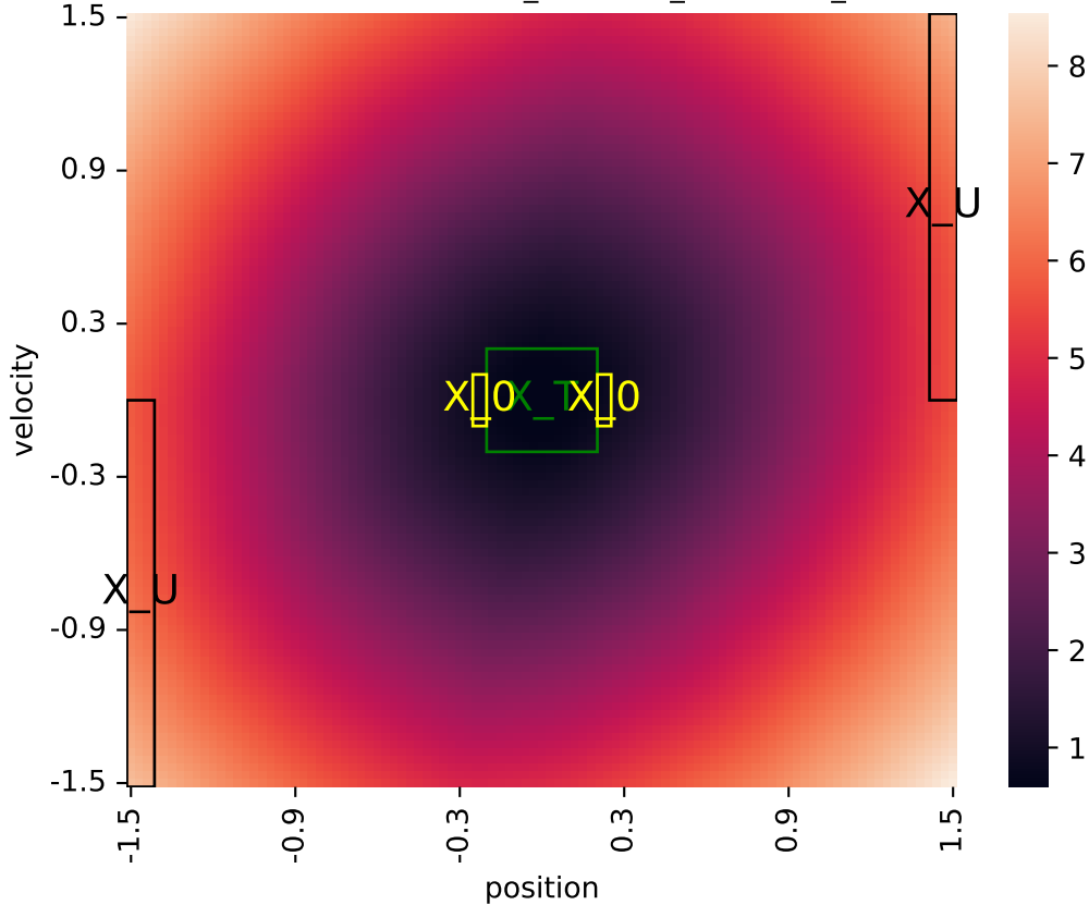
Learned certificate (2026-06-01_05-34-04_certificate_iteration=2)
