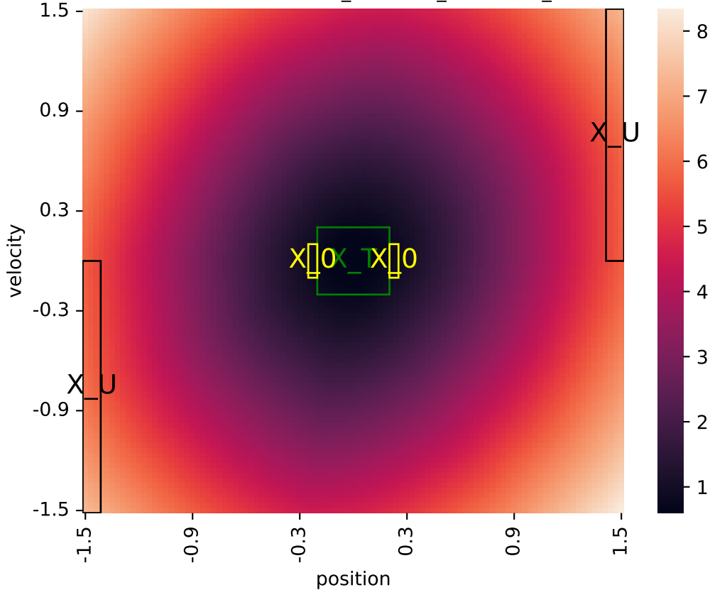
Learned certificate (2026-06-01_05-40-38_certificate_iteration=2)
