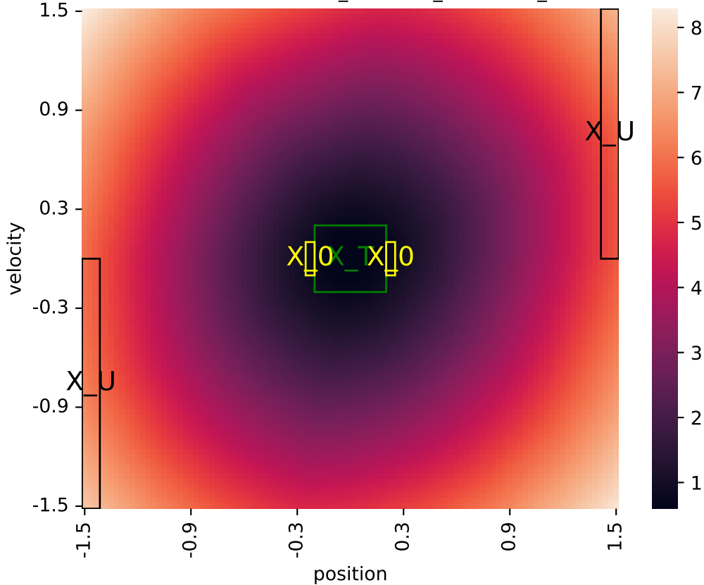
Learned certificate (2026-06-01_05-46-39_certificate_iteration=2)
