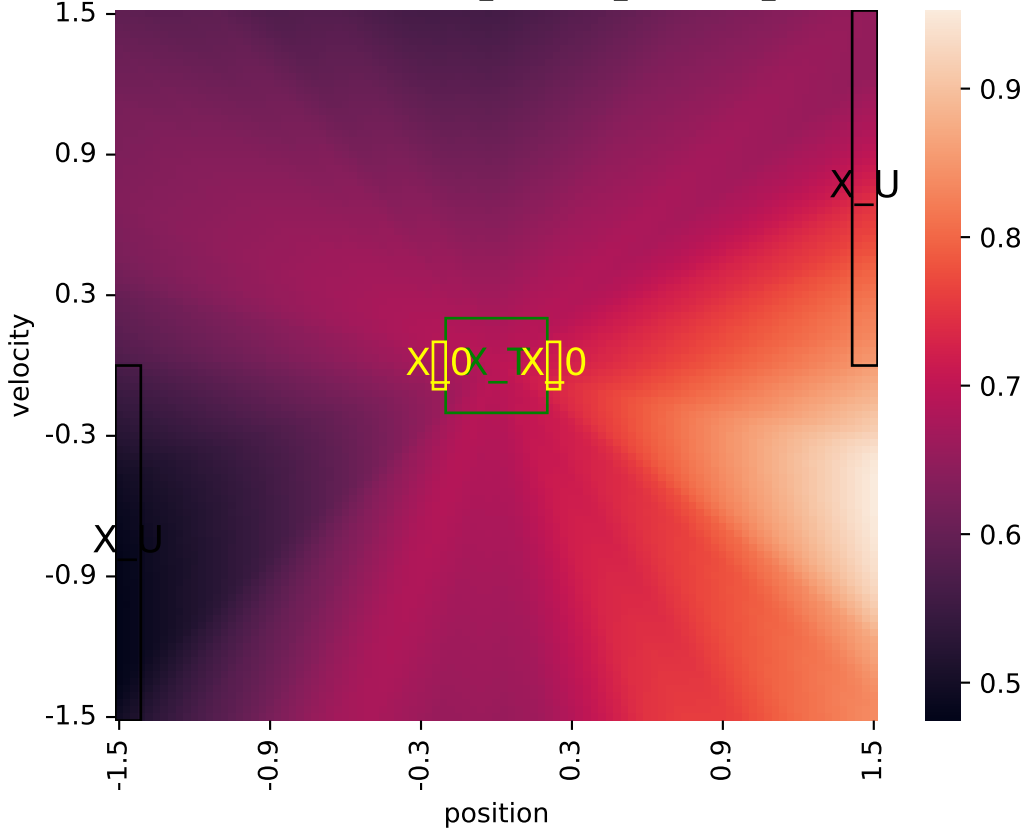
Learned certificate (2026-06-01_05-48-25_certificate_iteration=0)
