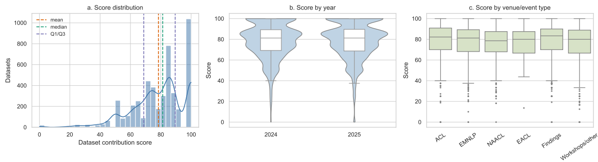
Figure 1: Score landscape.
