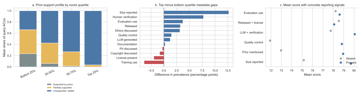
Figure 2: Score drivers.
