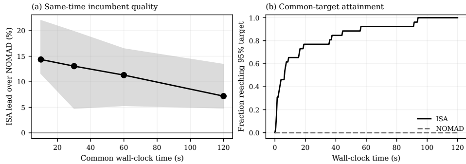
Figure 3 Anytime performance on 26 unique generated instances.
