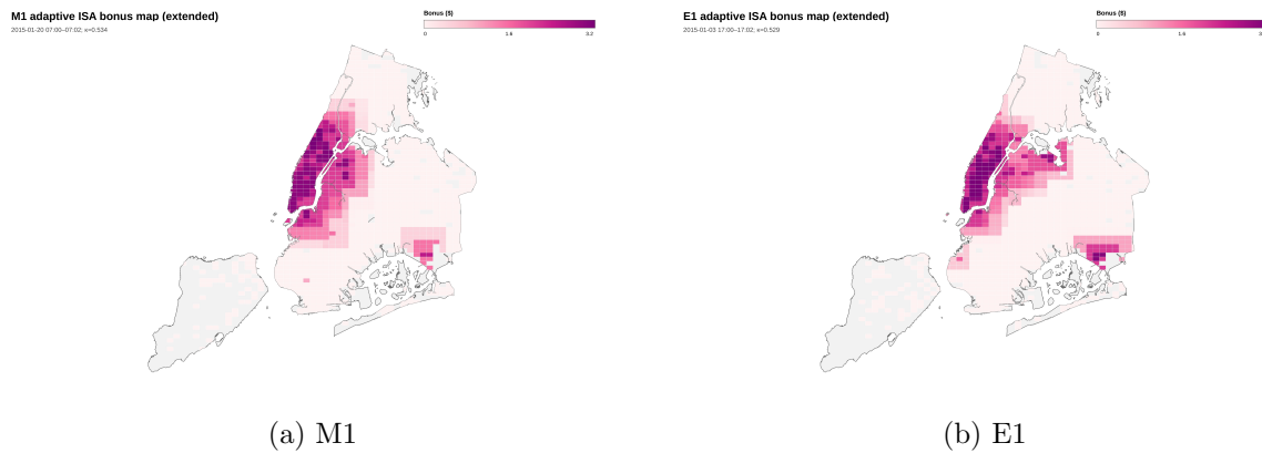
Figure 4 Optimized driver surge maps for two New York City instances.
