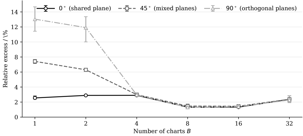
Figure 2 Decision quality as mode-specific scenario planes separate.
