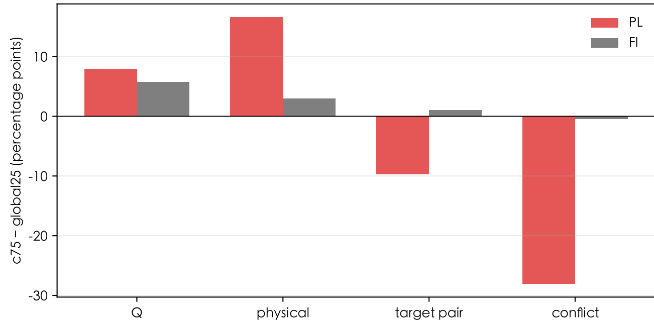
Conflict-specific effect after global-scale control
