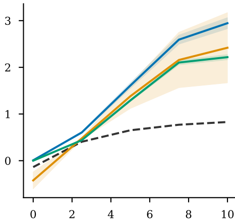
Latent Factor 2
