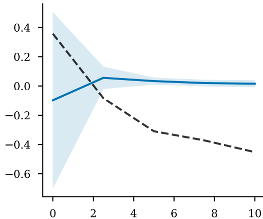
Latent Factor 2
