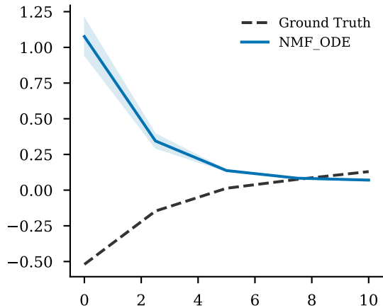
Latent Factor 1
