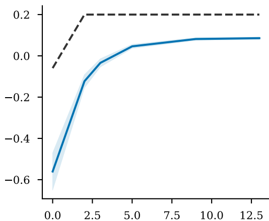
Latent Factor 2
