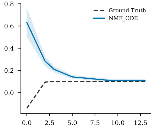
Latent Factor 1
