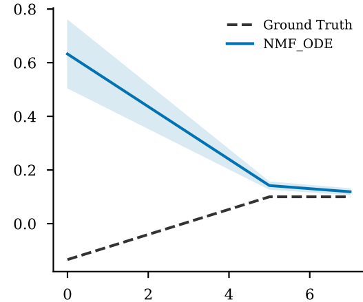
Latent Factor 1
