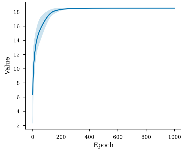
Likelihood
