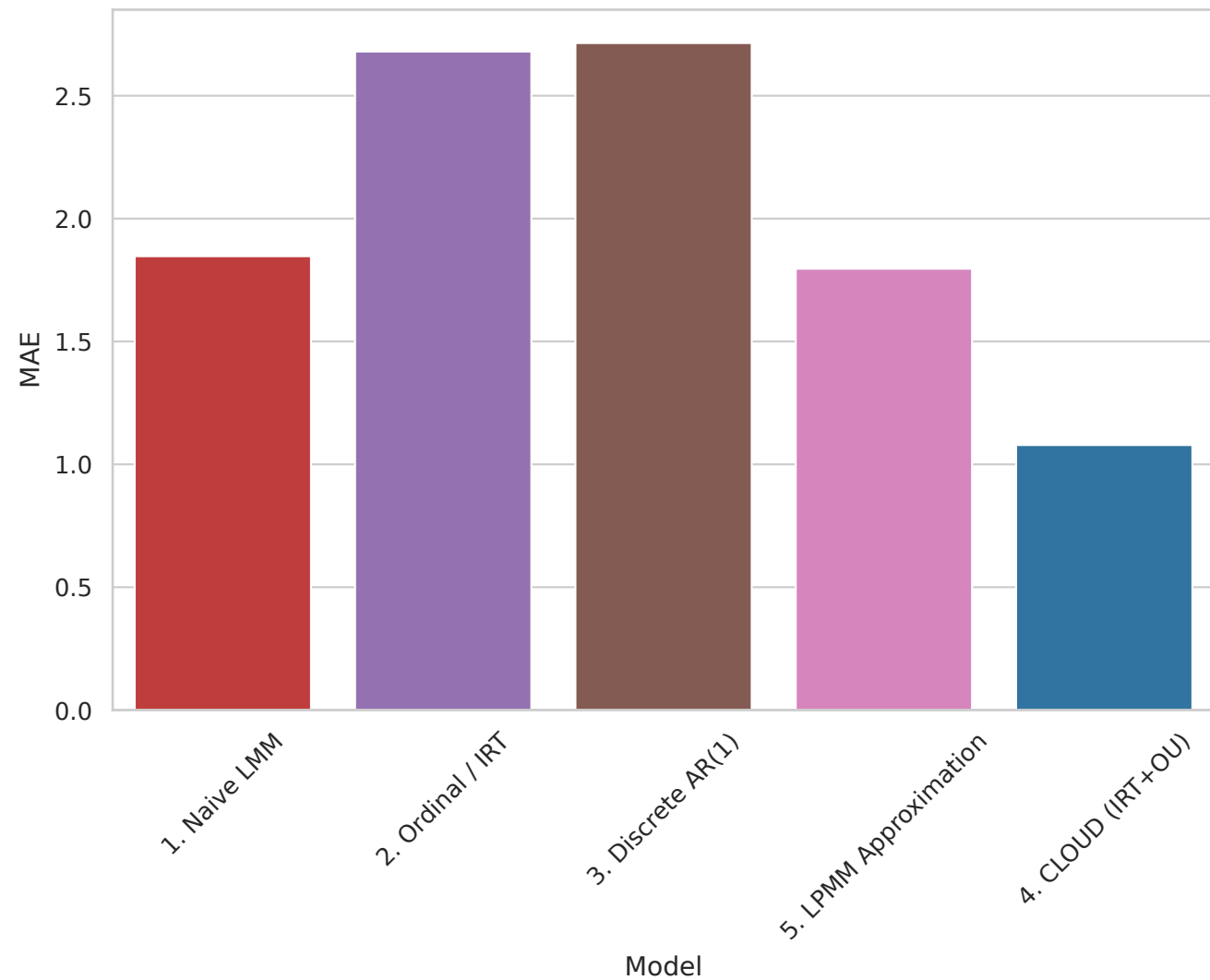
Total Score MAE
