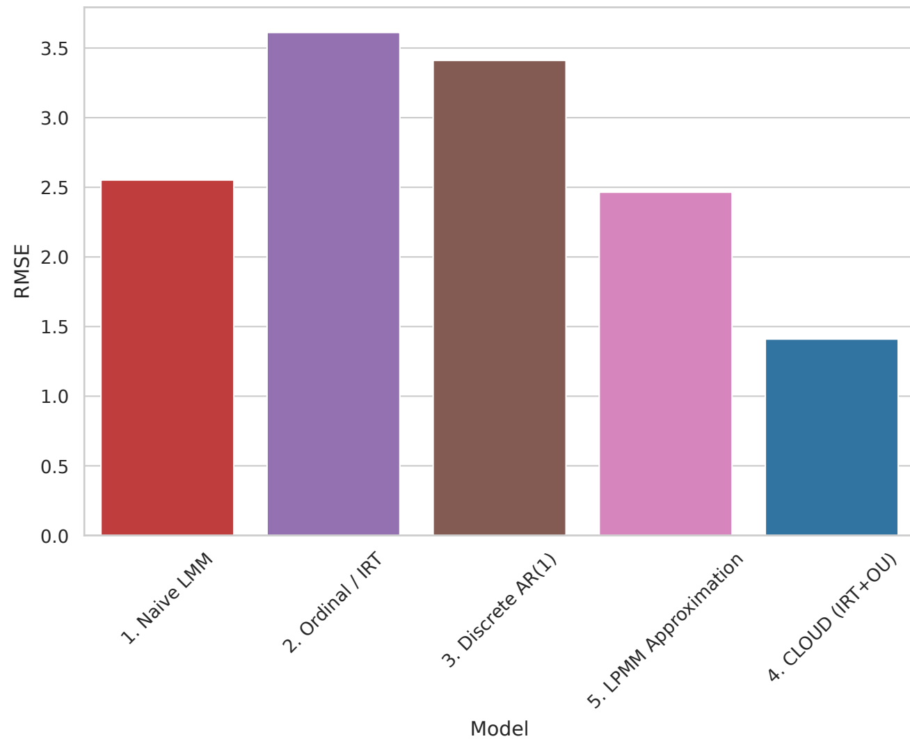
Total Score RMSE
