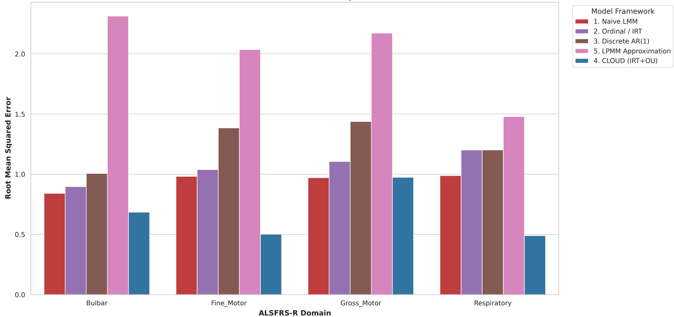
Domain-Level RMSE Comparison
