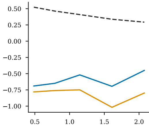
Latent Factor 3
