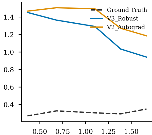
Latent Factor 1
