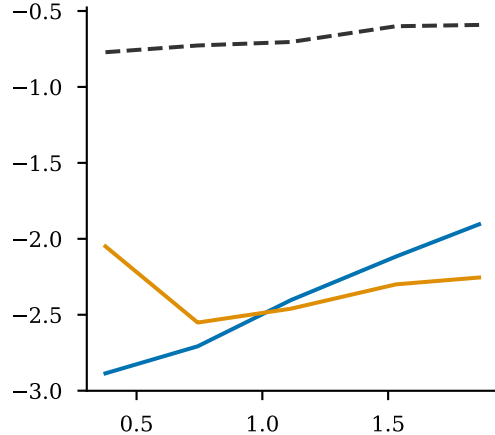
Latent Factor 3
