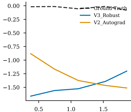
Latent Factor 1
