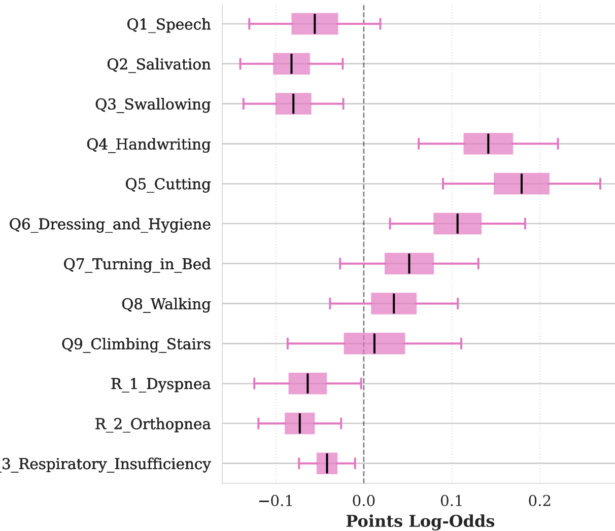
1. Naive LMM
