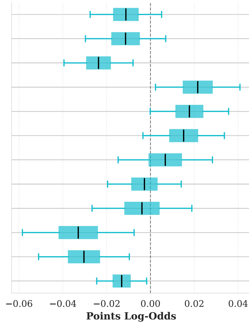
3. Univariate CAR(1)
