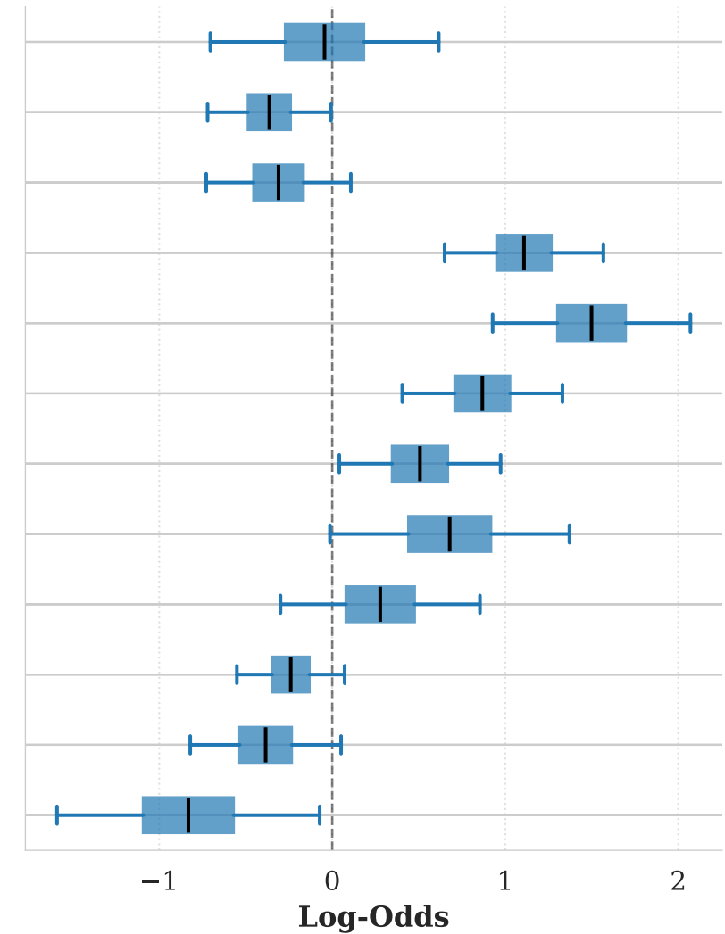
4. CLOUD
