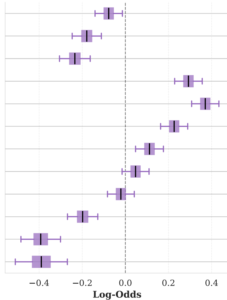
2. LPMM Approximation
