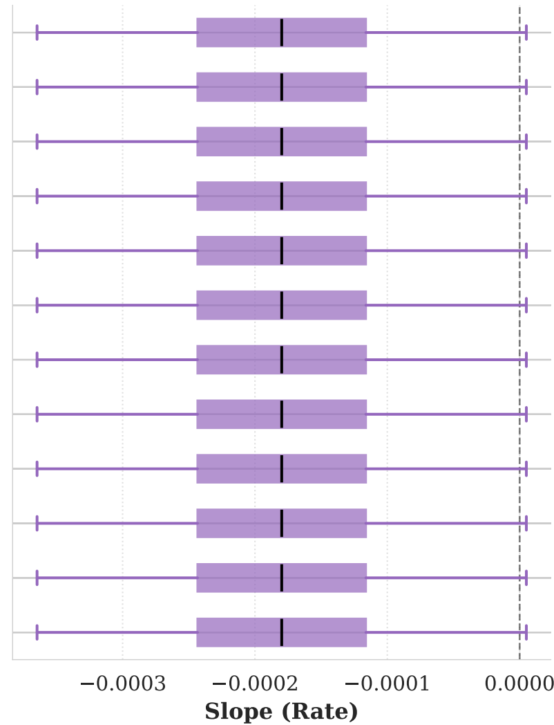
2. LPMM Approximation
