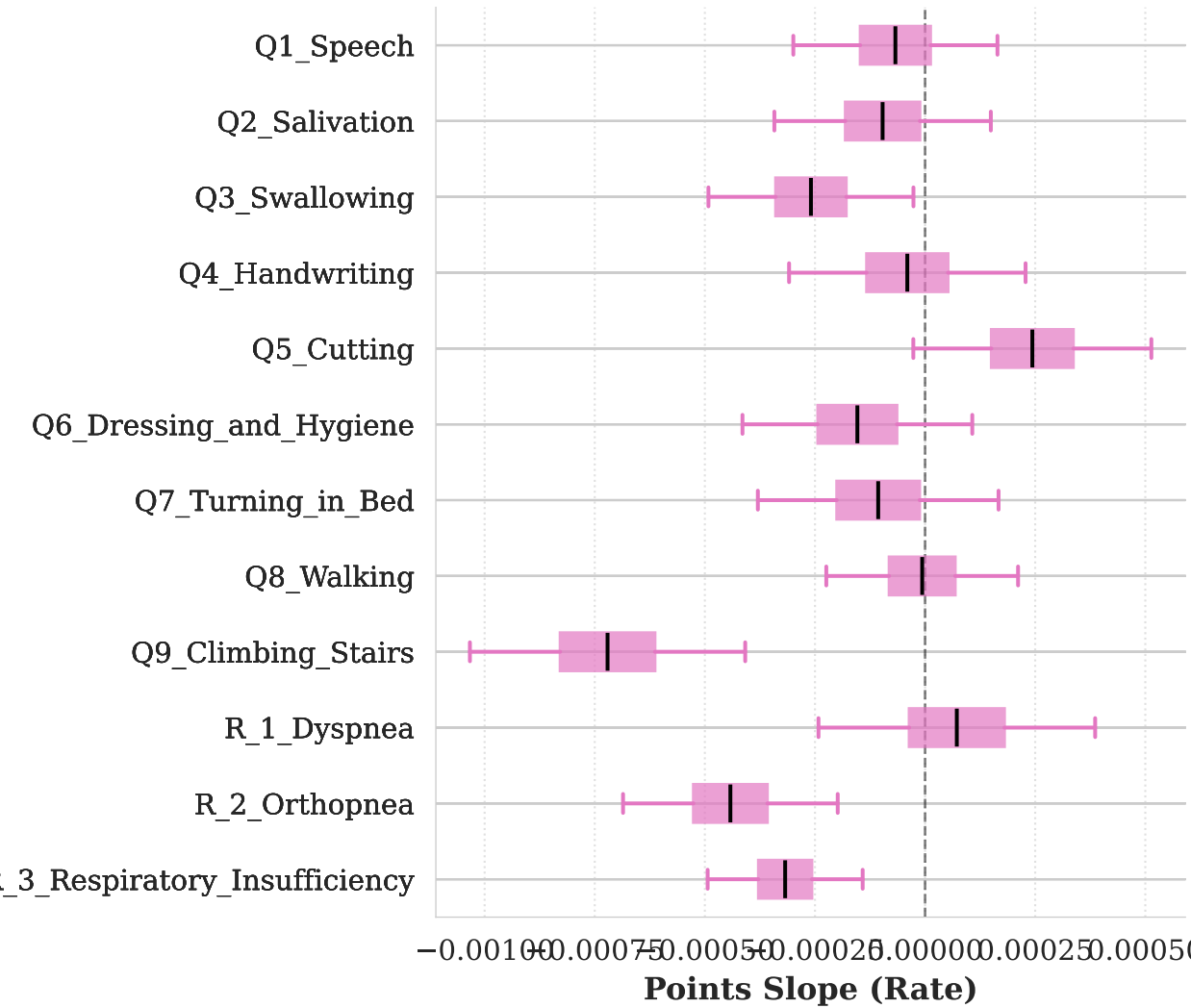
1. Naive LMM
