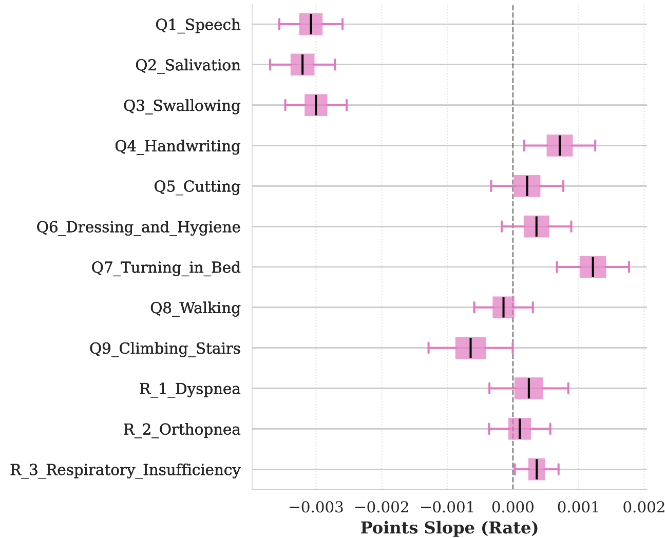
1. Naive LMM
