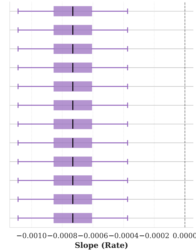
2. LPMM Approximation
