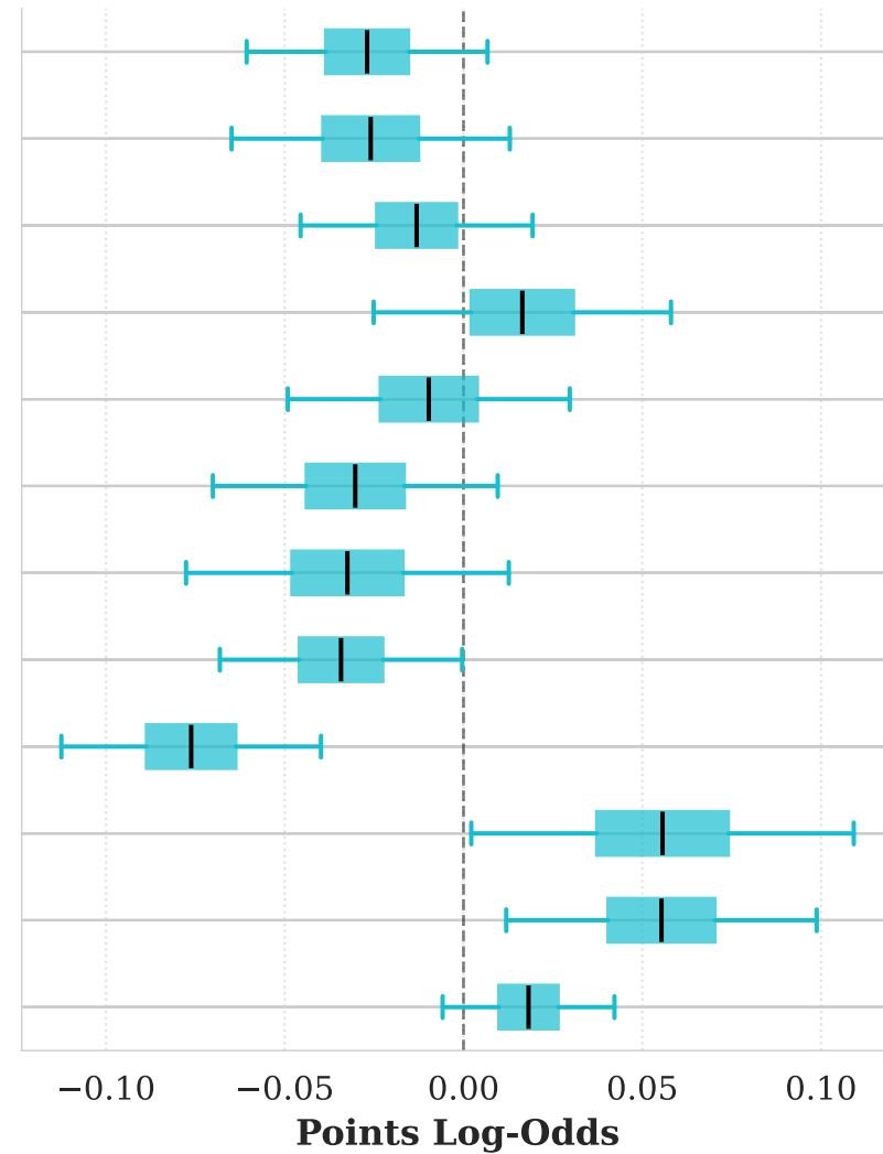
3. Univariate CAR(1)
