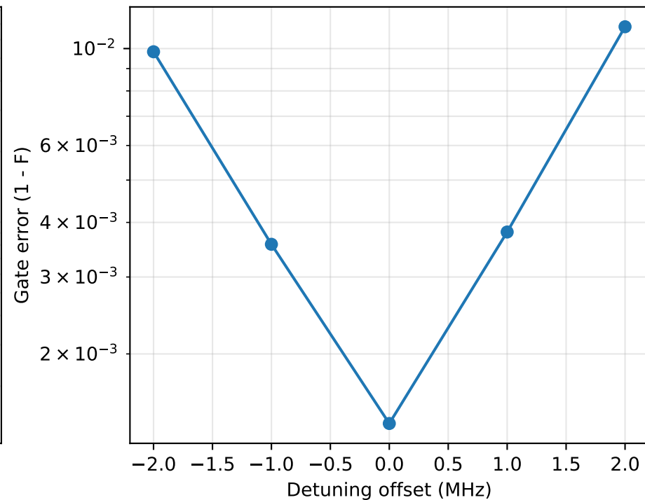
CZ sensitivity (noise), tg=91.948 ns, n_truc=60, T1/Tphi=30 us
