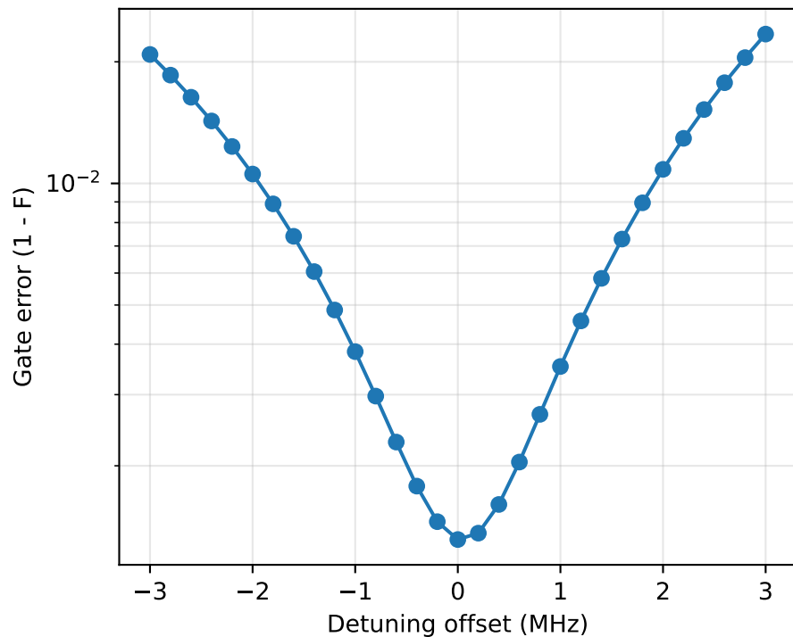
CZ sensitivity (ideal), t_g=91.948 ns, n_{\text{truc}}=300
