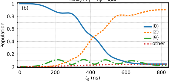
Noisy, T_1 = T_\phi = 3\mu s
