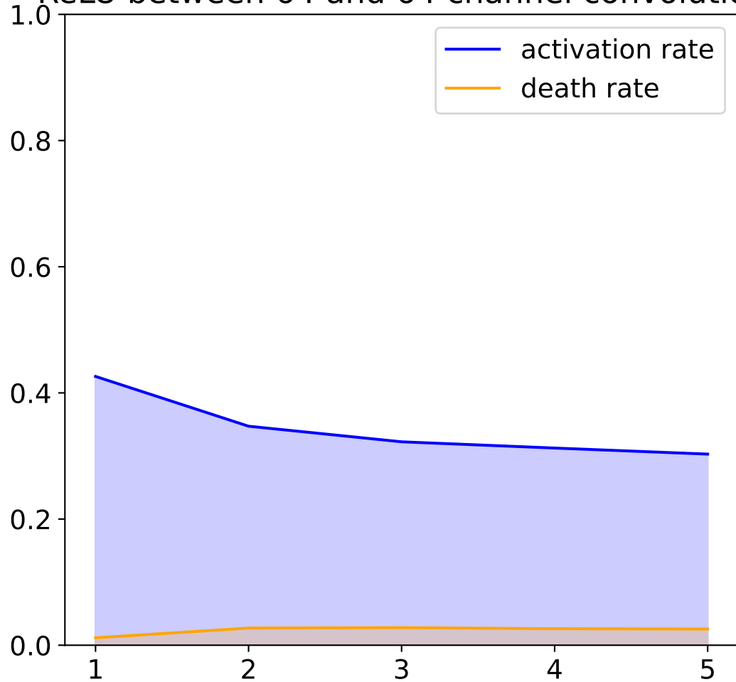
ReLU between 64 and 64 channel convolution
