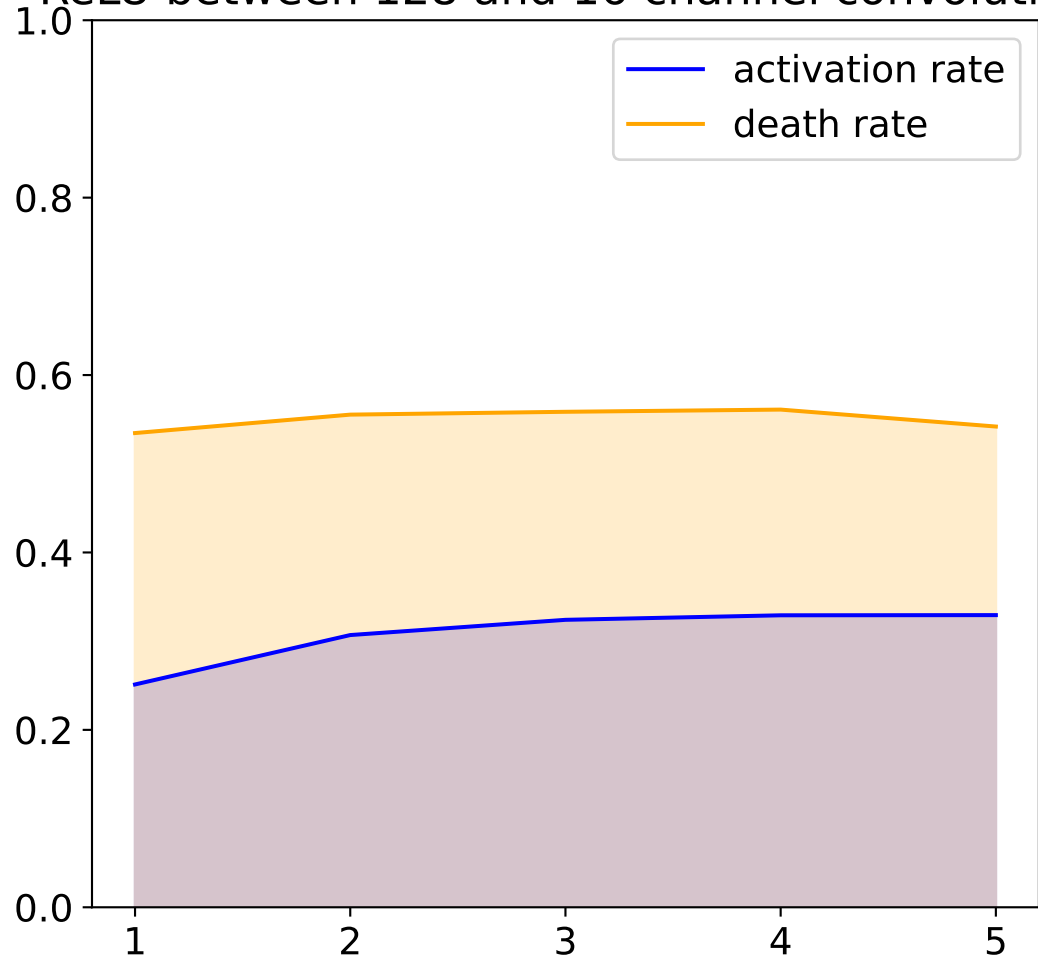
ReLU between 128 and 16 channel convolution
