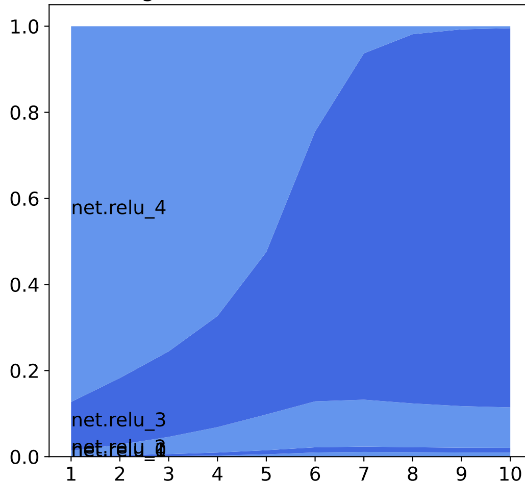
Weights Initialized Uniform (-1, 1)
