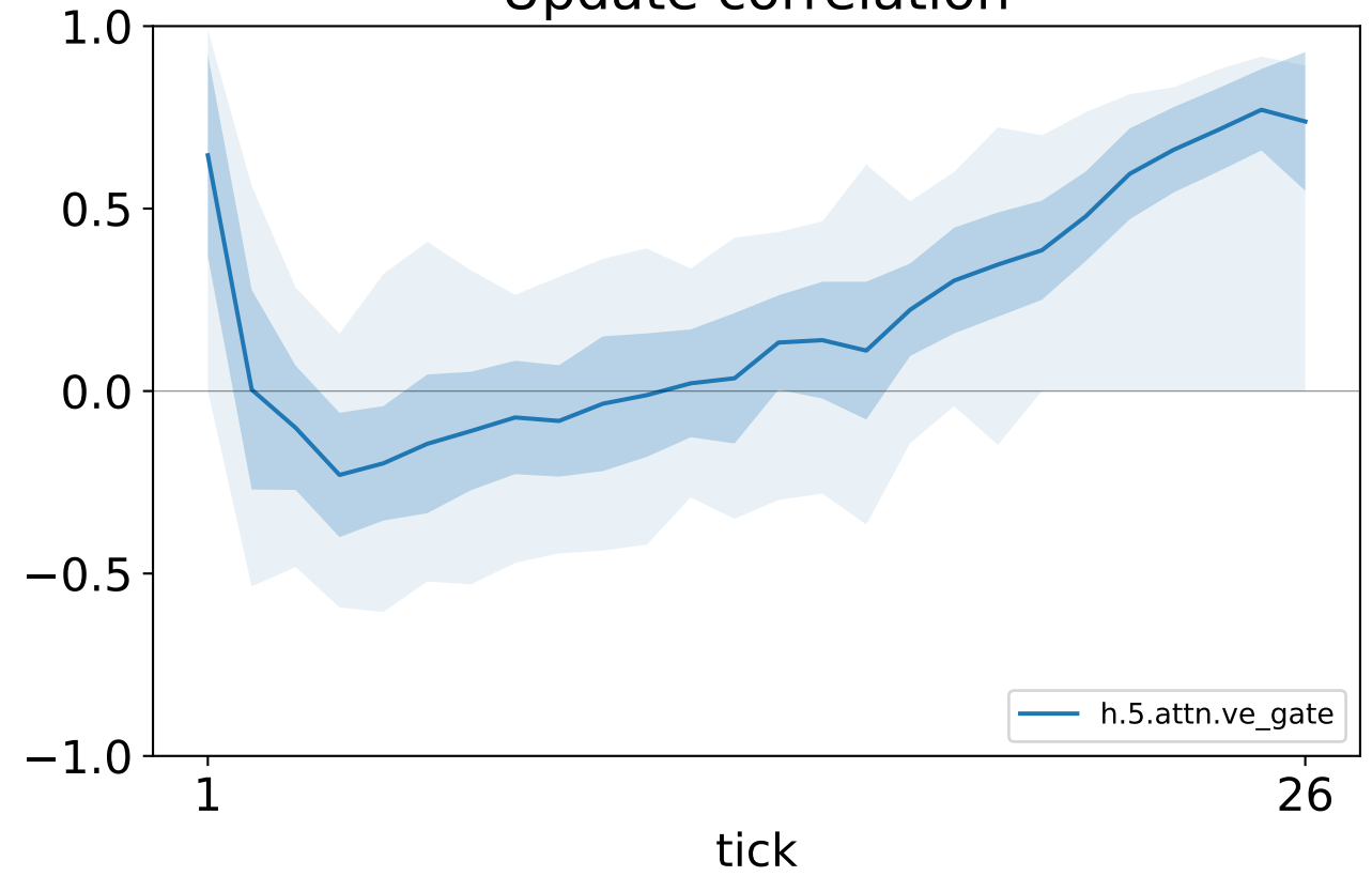
Update correlation
