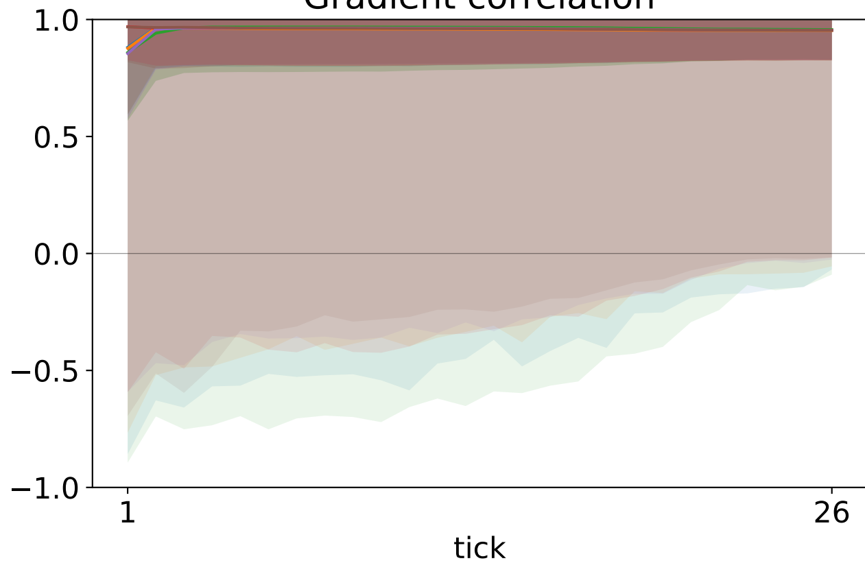
Gradient correlation
