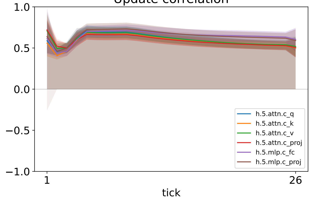
Update correlation
