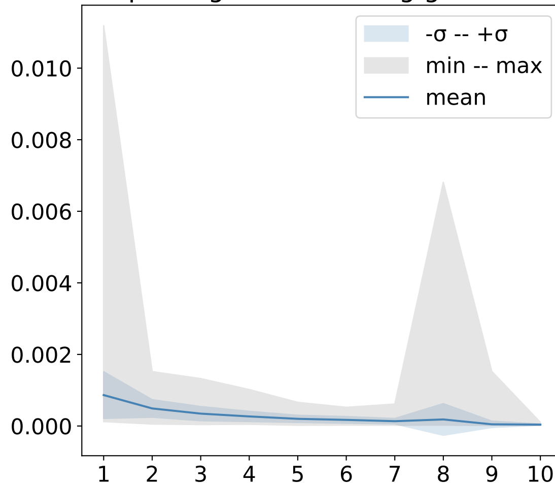
Exploding and Vanishing gradients
