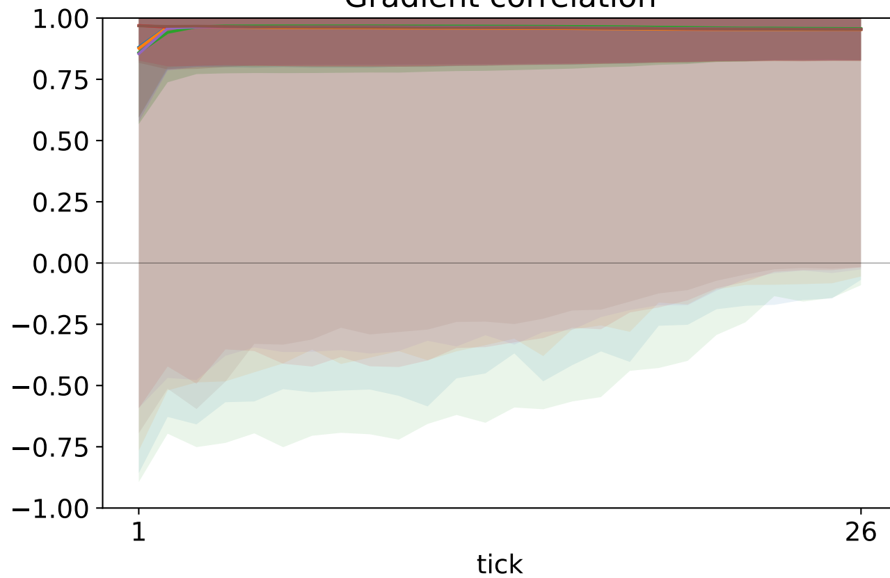
Gradient correlation
