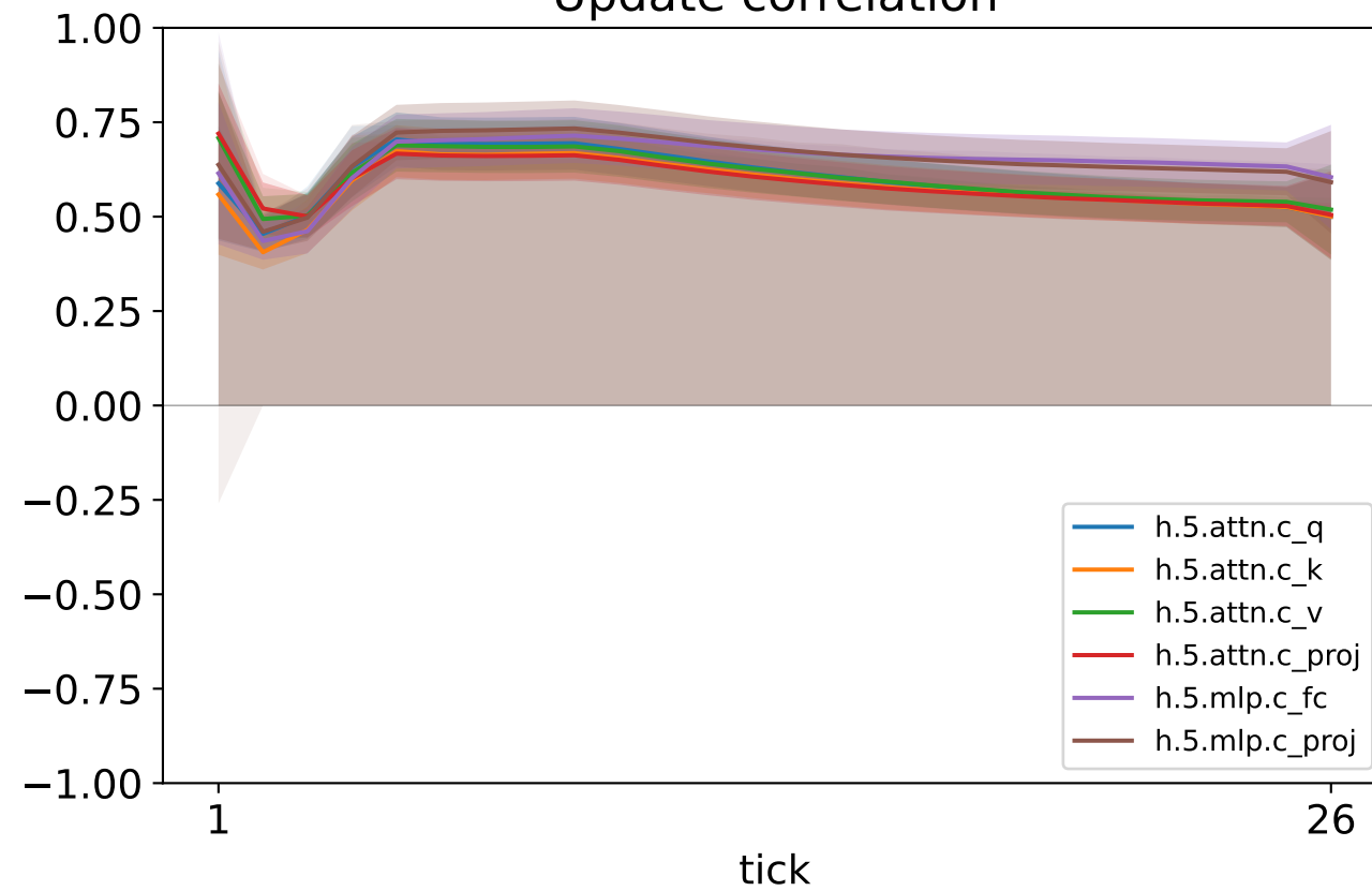
Update correlation
