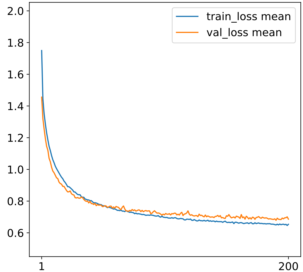
Loss curves
