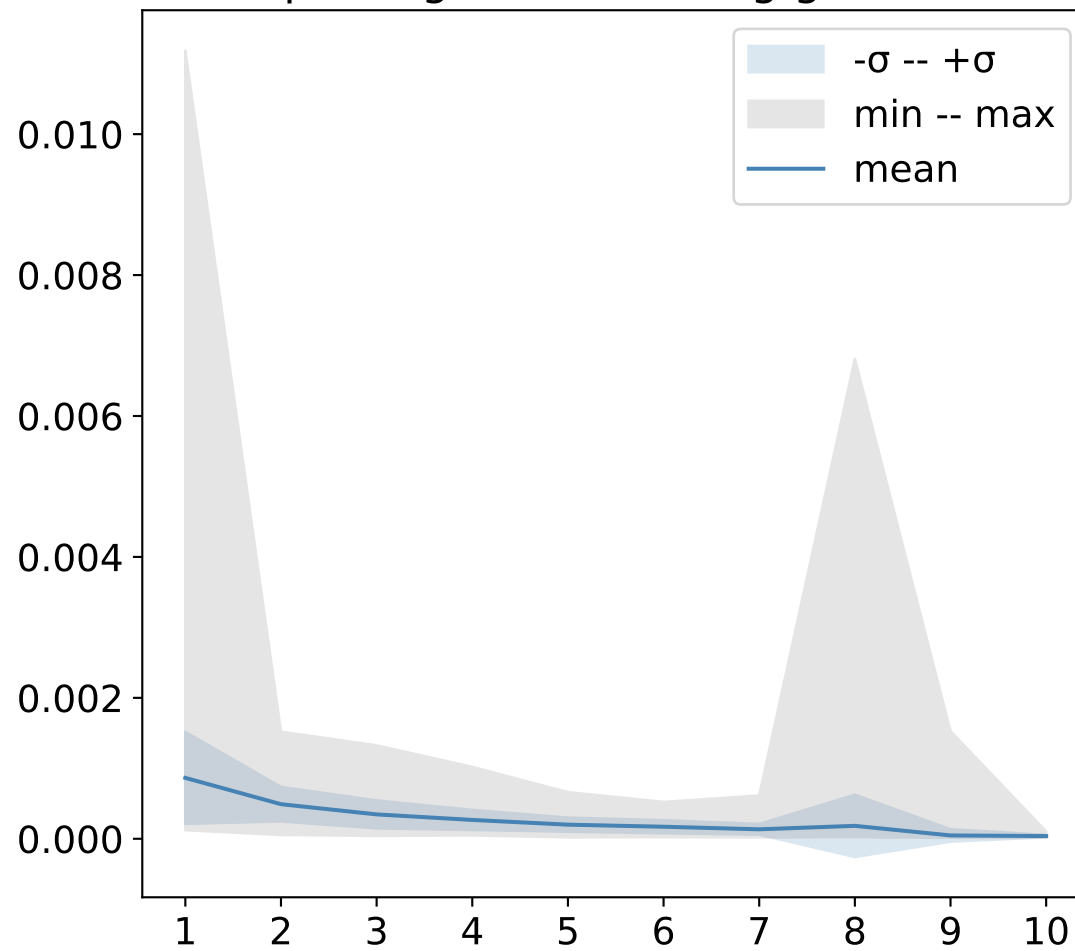
Exploding and Vanishing gradients
