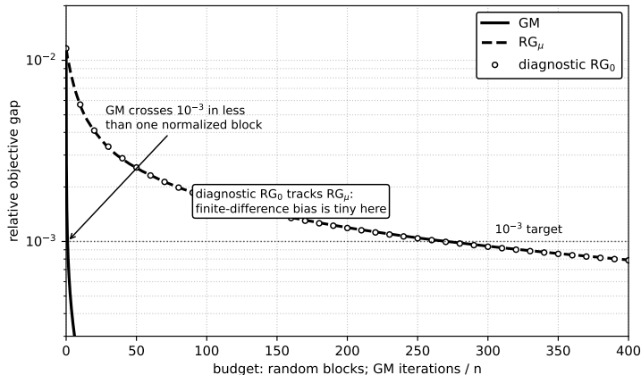
Smooth quadratic chain, n=64 , mean over 10 seeds
