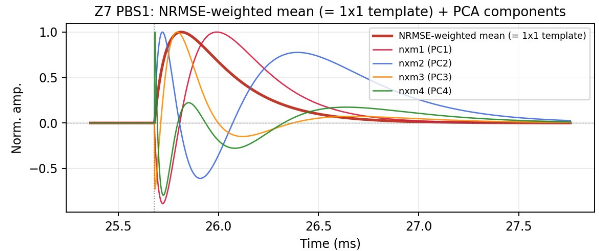
NxM with the NRMSE-weighted mean (= 1x1) + the same \text{nxm1} – 4
