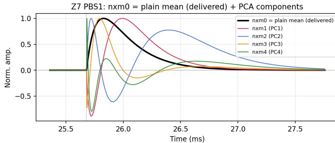
NxM with the plain mean: \text{nxm0} (delivered) + \text{nxm1} – 4
