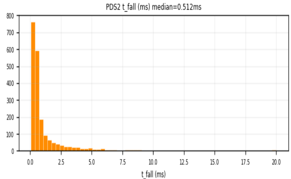
Z7 PDS2 alone, fitted \tau_{\text{fall}} : broad tail (median 0.51 ms vs \approx 0.25 ms on good channels) — the artifact quantified
