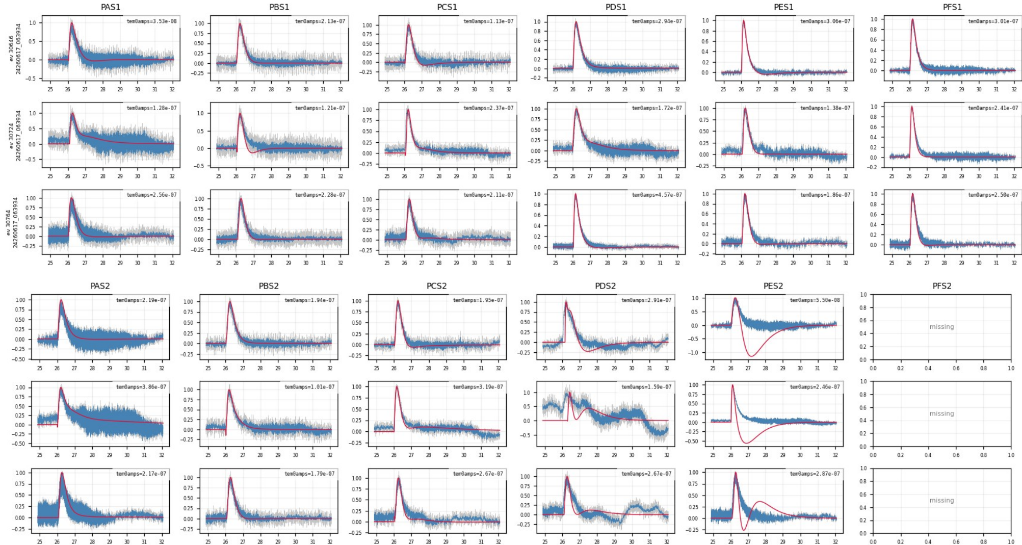
Z7, 3 example K-line events (top: S1 channels, bottom: S2): raw (gray) / LP (blue) vs \sum \text{amp}_k \cdot \text{nxm}_k (red), amplitudes from the UMN (Addison) processing of our templates
