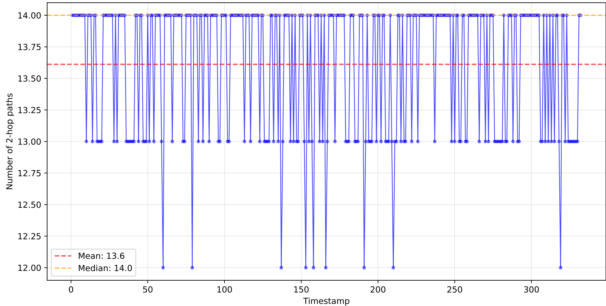
2-hop paths between 10.1.1.100 and 10.1.1.102 in Period 2
