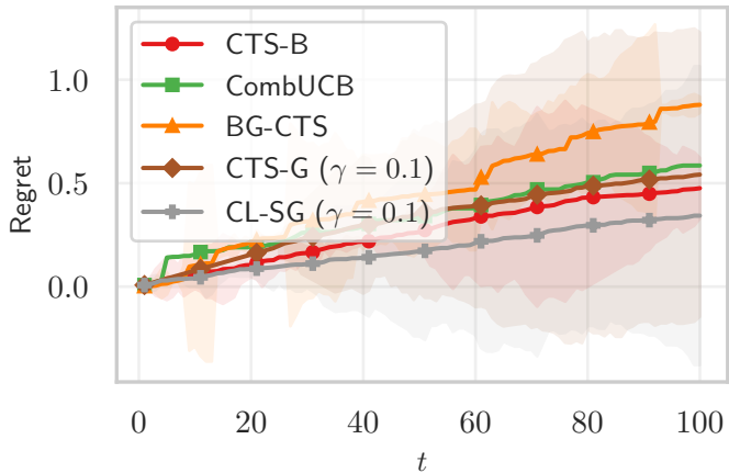
Algorithm Comparison
