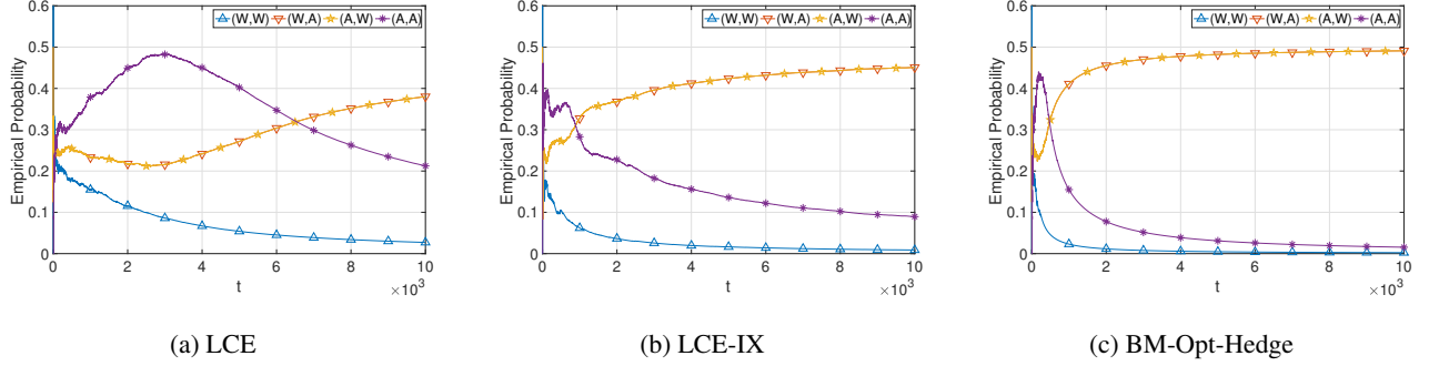
Figure 3: The empirical distribution of joint actions by two agents in T rounds.
