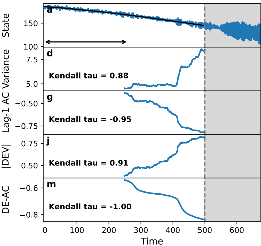
Fox model
