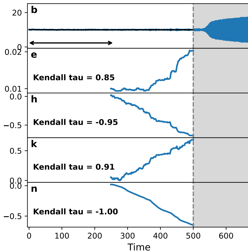
Ricker model
