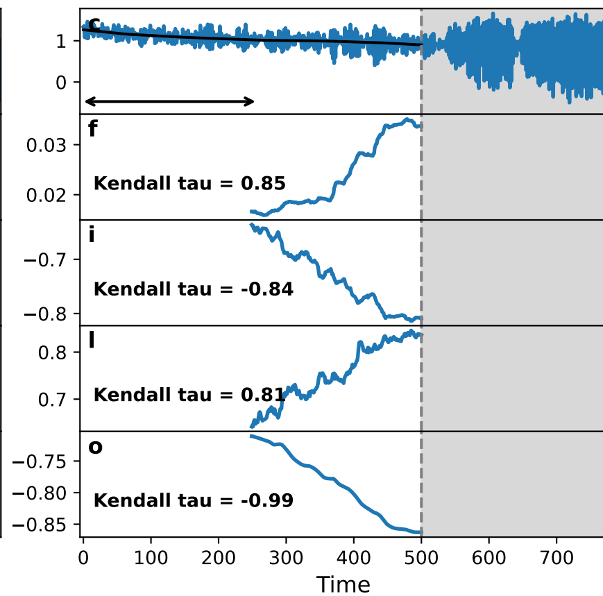
Henon map model
