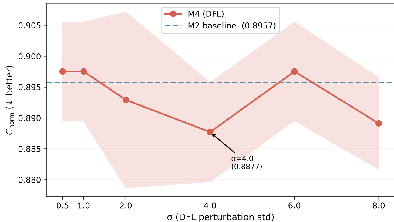
M4 DFL Performance vs. Perturbation Scale \sigma (mean \pm std across seeds 42/43/44)
