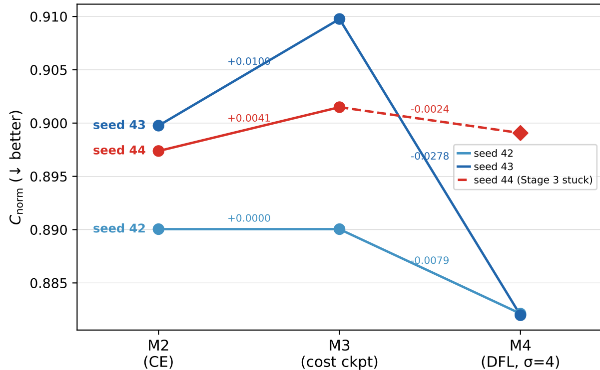
Per-Seed: M2 \rightarrow M3 \rightarrow M4 \sigma=4.0 (dashed + \blacklozenge = Stage 3 did not improve)
