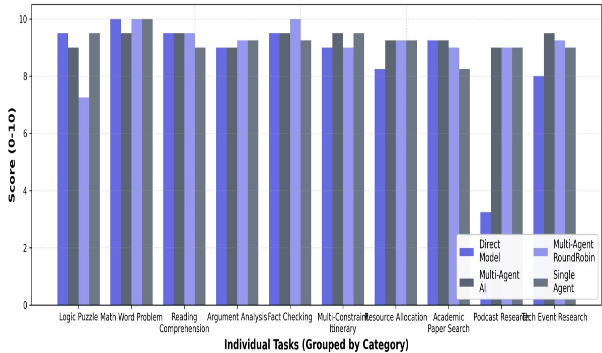
Performance by Individual Task
