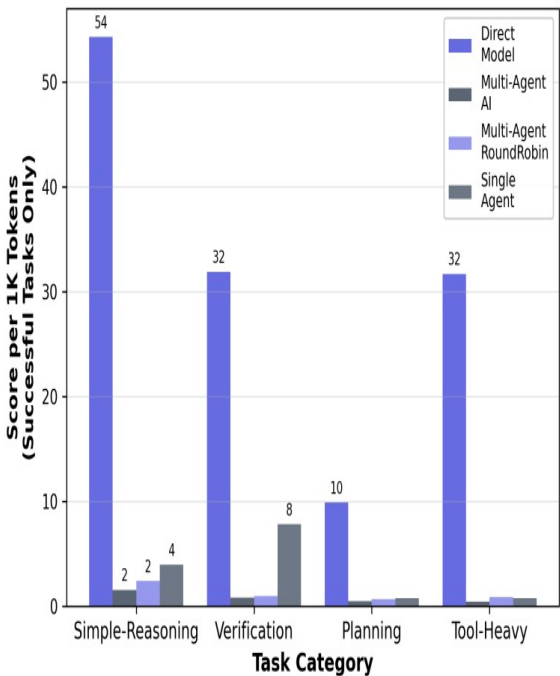
Token Efficiency by Task
