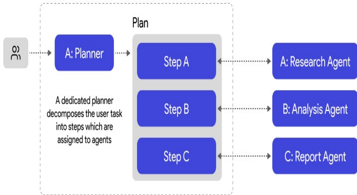
Figure 2.6: Plan-Based Orchestration Pattern showing a single orchestrator managing task execution across multiple agents.
