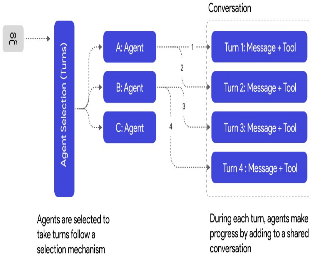
Figure 2.8: In conversation-Driven patterns, agents primarily collaborate by appending to a shared conversation.
