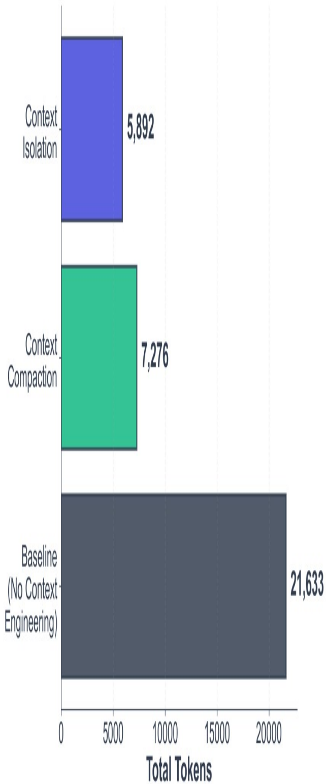
Total Token Usage
