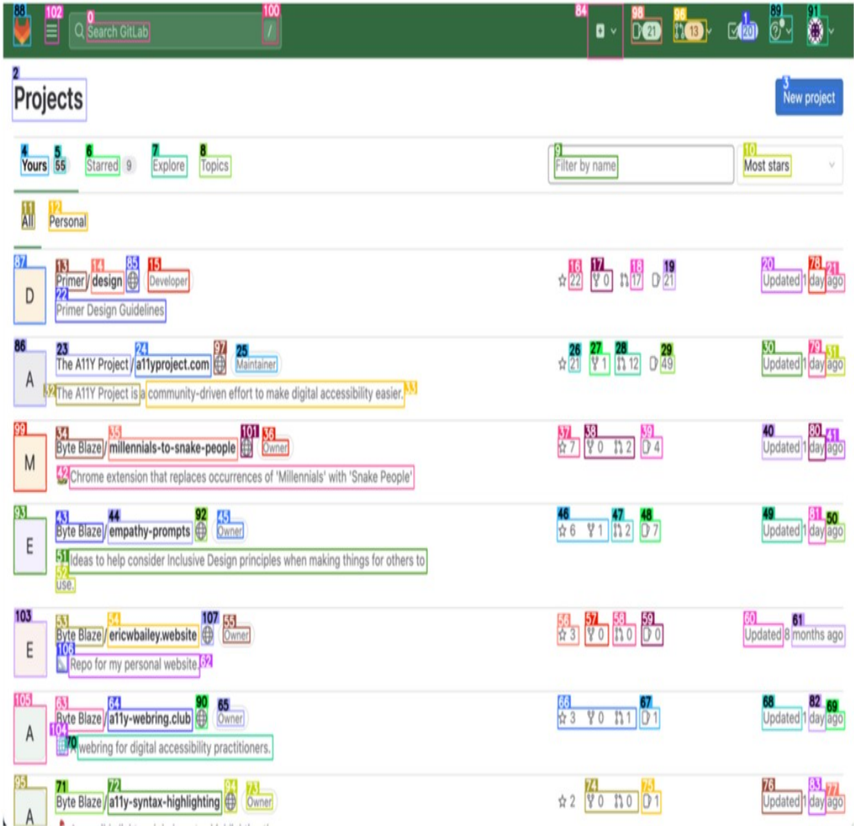
Figure 5.3: OMNIPARSER applies a detection model to parse interactable regions on the screen and a caption model to extract the functional semantics of the detected elements used to annotate the image before being passed to a generative model for action generation.
