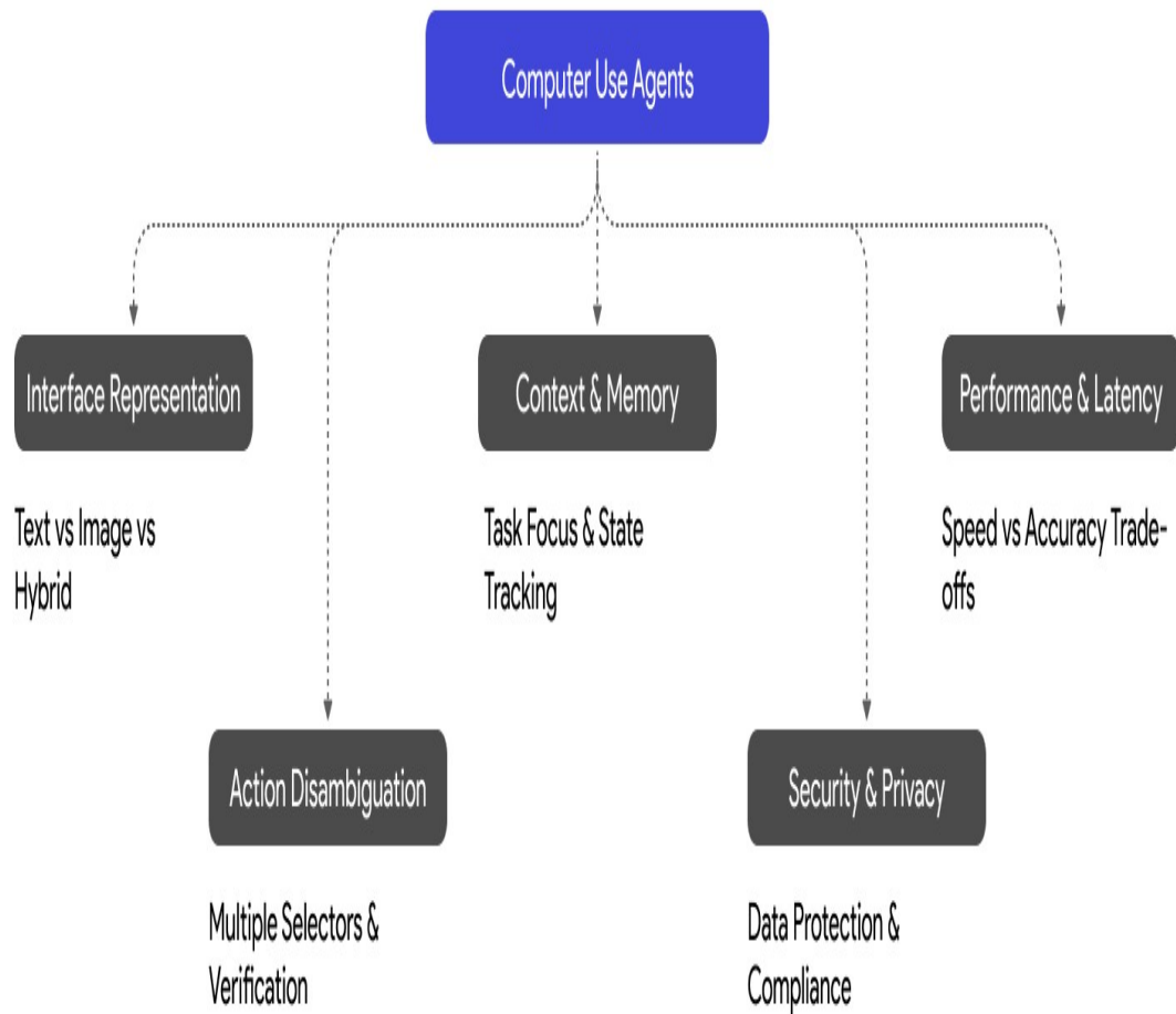
Figure 5.4: Key challenges in implementing computer use agents. The diagram illustrates five major hurdles: interface representation (balancing detail and efficiency), context and memory management (maintaining task relevance), action disambiguation (resolving ambiguous targets), security and privacy (protecting sensitive data), and latency (balancing speed and accuracy). These interconnected challenges highlight the complexity of developing effective and reliable computer use agents for real-world applications.
