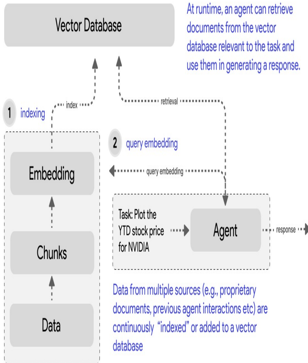
Figure 4.2: Long-term memory uses vector databases to store and retrieve vast amounts of information through RAG (Retrieval-Augmented Generation). Data is indexed as embeddings, and at runtime, agents query the database to retrieve relevant context for generating responses.
