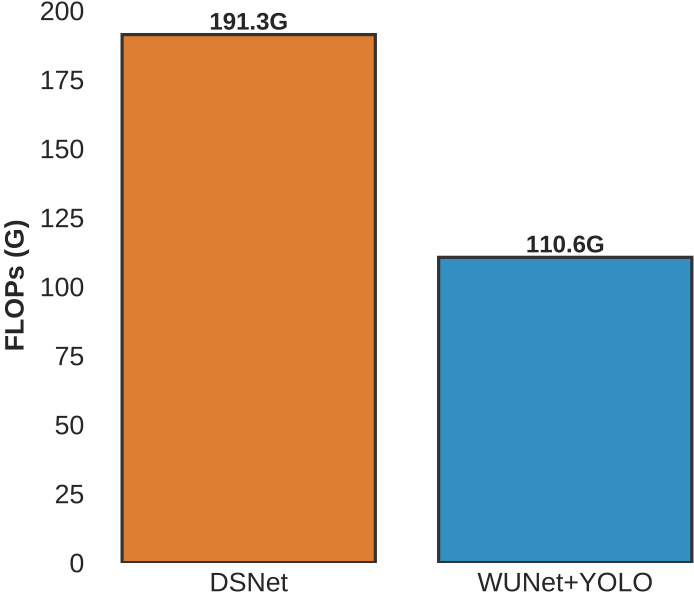
FLOPs Comparison
