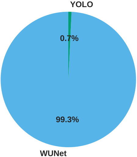
WUNet+YOLO Latency Distribution
