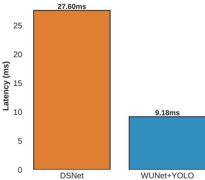
Latency Comparison
