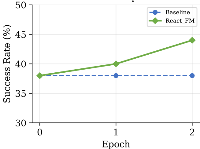
WebShop
