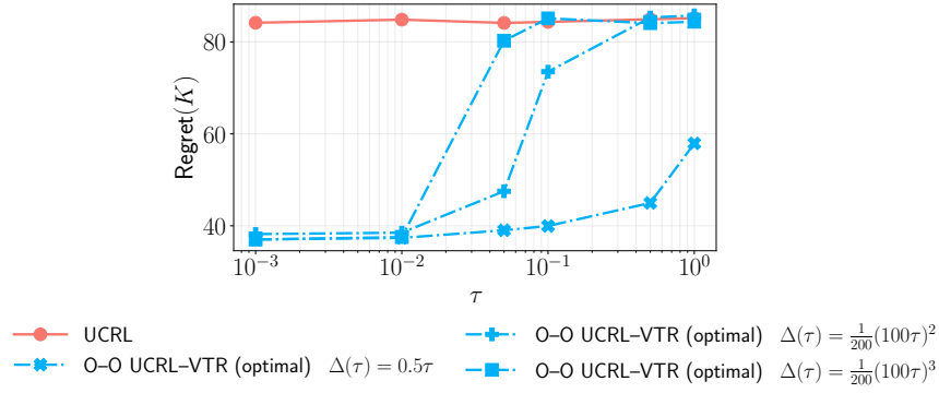
Figure 3 Cumulative regret versus \tau for different \Delta(\tau) , with K = 4 \times 10^3 and M^{\text{off}} = 10^5 .
