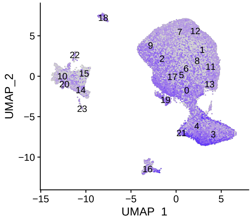
PLP1
