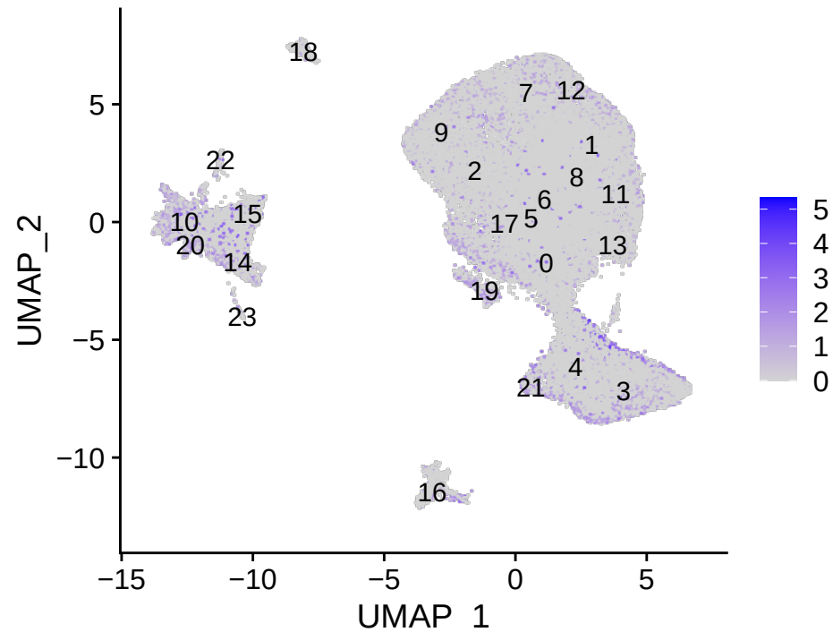
CNP
