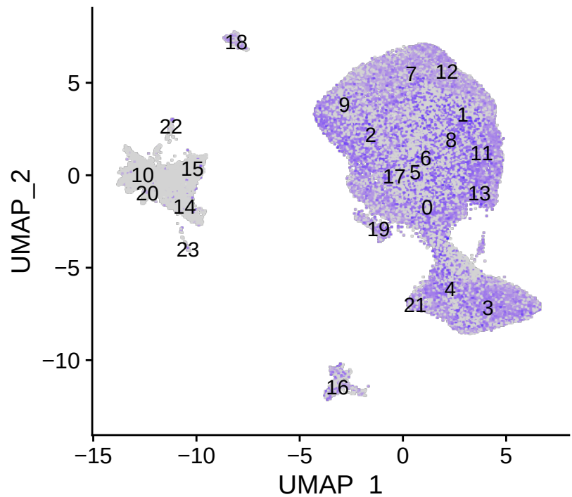
SOX6
