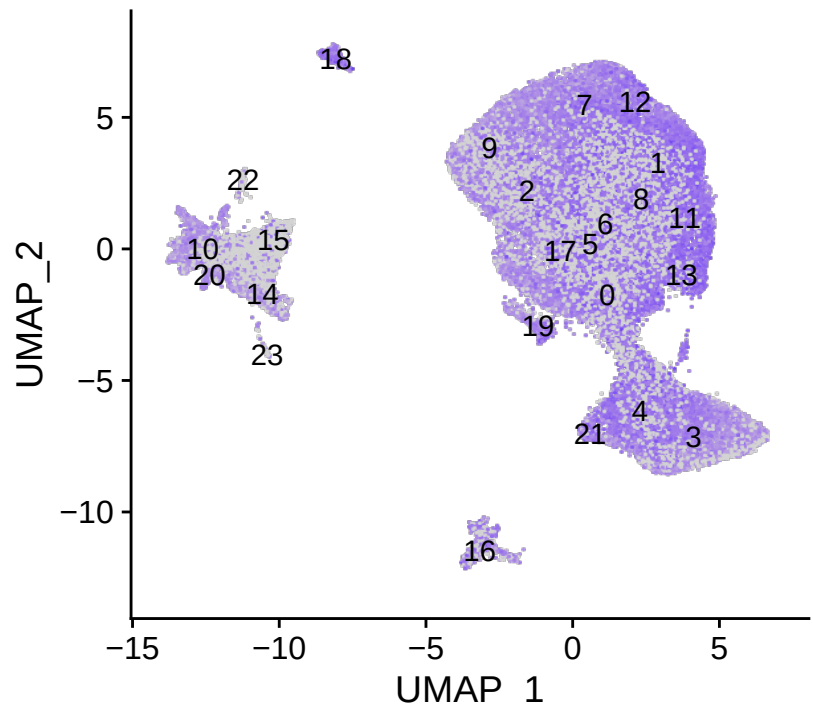
HSP90AA1
