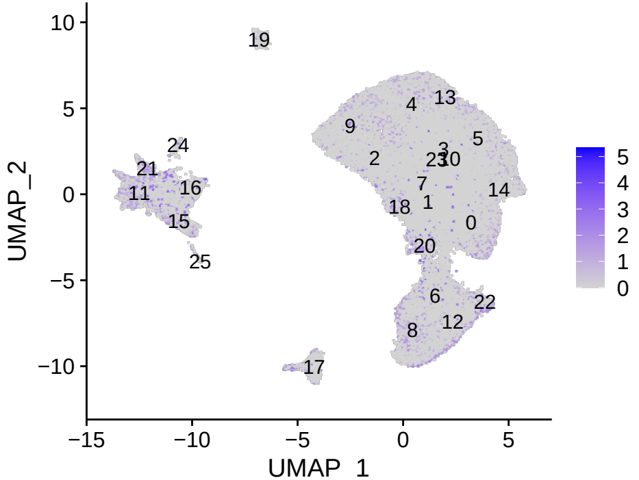
CNP
