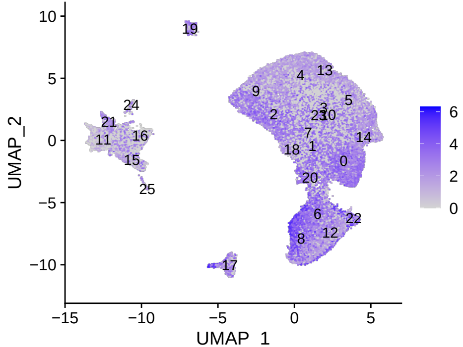
PLP1
