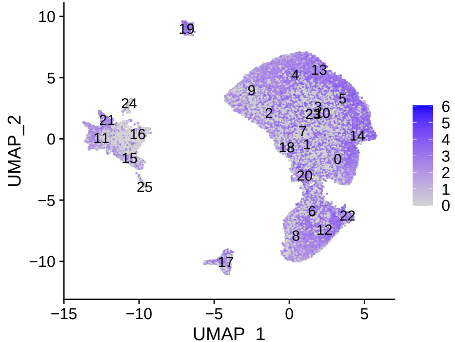
HSP90AA1
