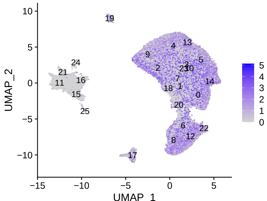
SOX6
